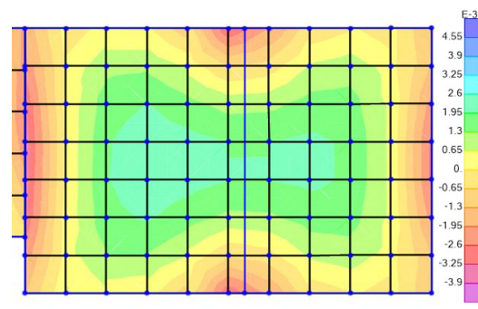
Fig. 3b: With Hidden Beam
