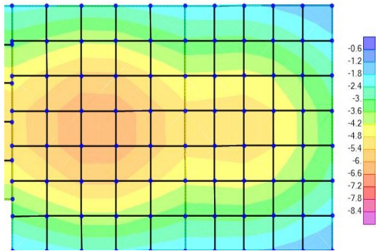
Fig. 2a: With Drop Down Beam
