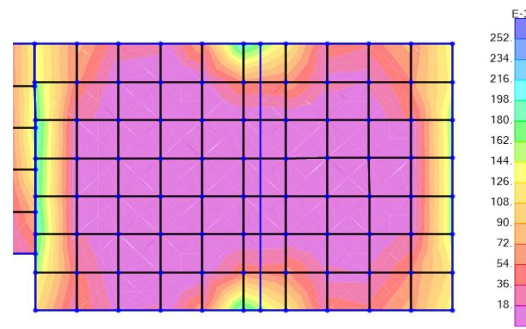
Figure 4b: With Hidden Beam
