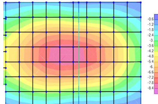
Fig. 2b: With Hidden Beam
