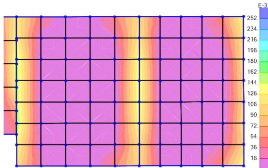
Figure 4a: With Drop Down Beam
